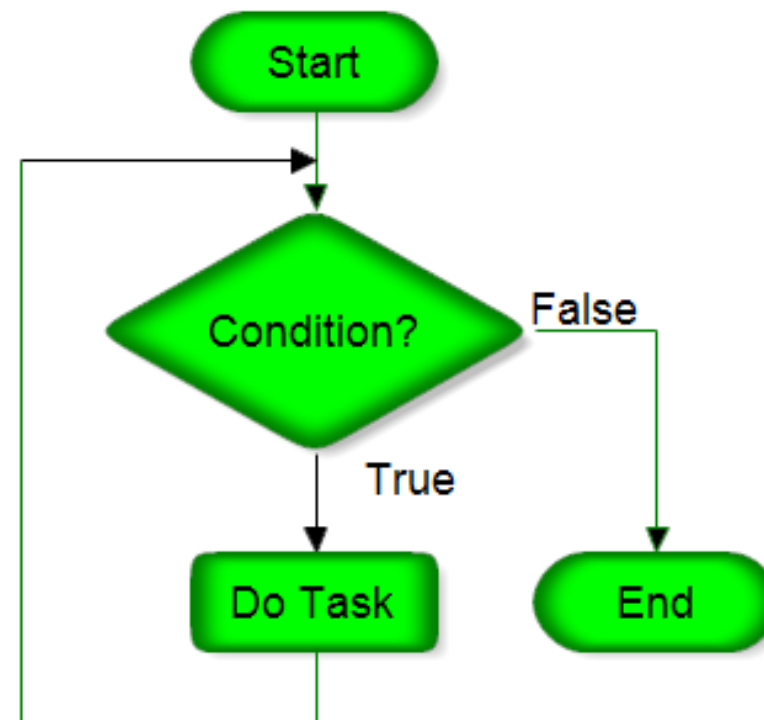
While Loop
